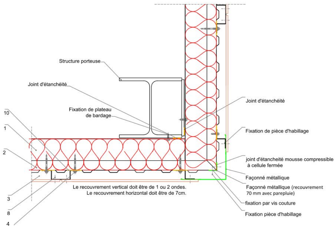
Figure 20 – Angle sortant – Coupe horizontale
