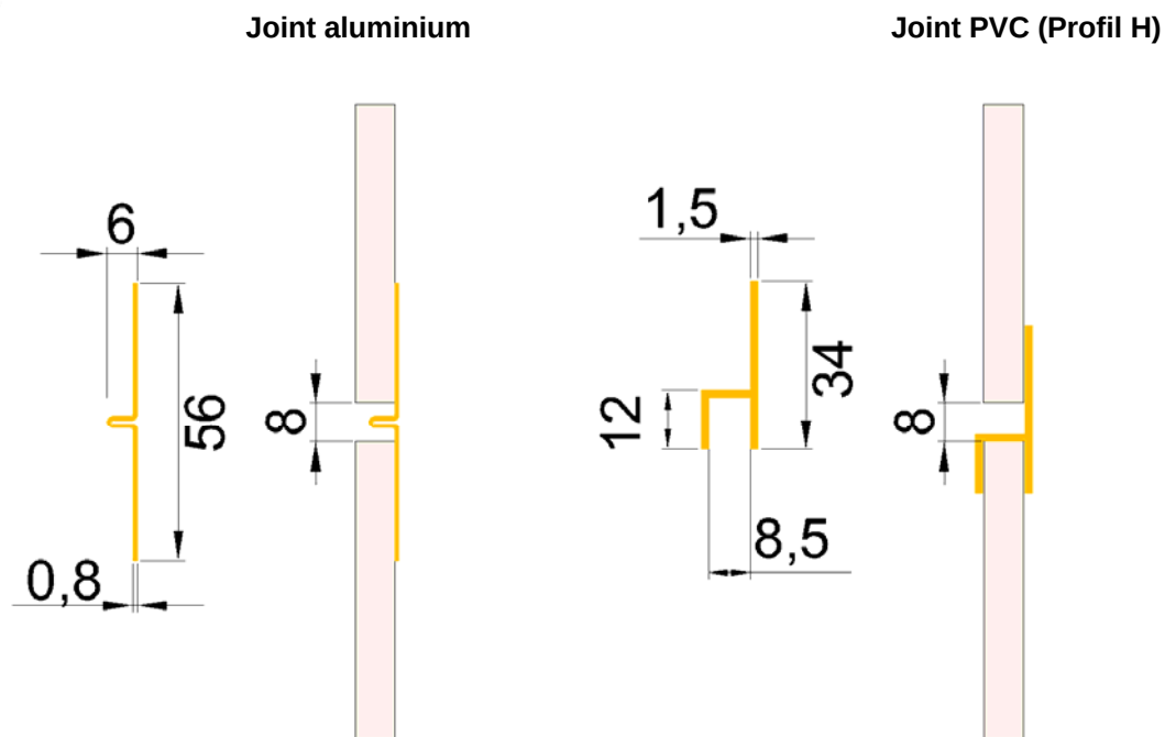
Figure 5 - Exemple de joint horizontal
