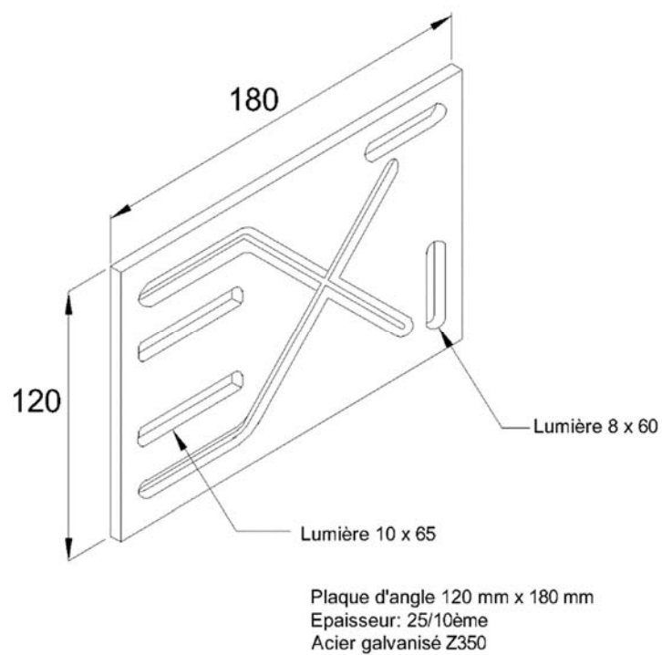
Figure 11 – Plaque d'angle ETANCO
