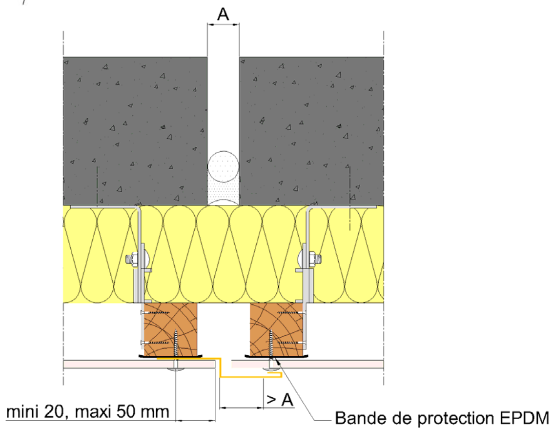
Figure 17 - Joint de dilatation
